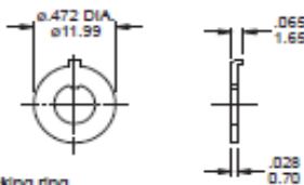
Locking ring supplied with B8 bushing
