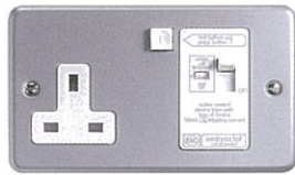
K6102 ALM 1 Gang 13A RCD Protected 10mA Tripping Current For Active Control Circuit
