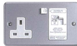
K6302 ALM 1 Gang 13A RCD Protected 30mA Tripping Current For Active Control Circuit
