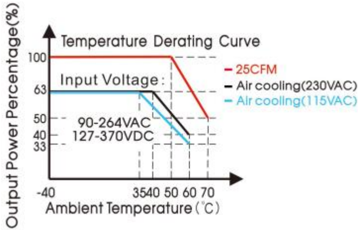
2367917 (full load 450W with 25CFM)
