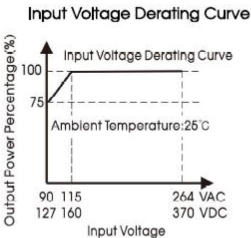
2367914, 2367917 Input Voltage Derating Curve
