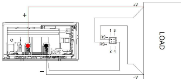
Remote sensing function wiring diagram
