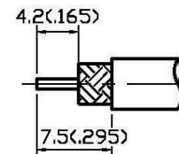
STRIPPING DIMENSION
