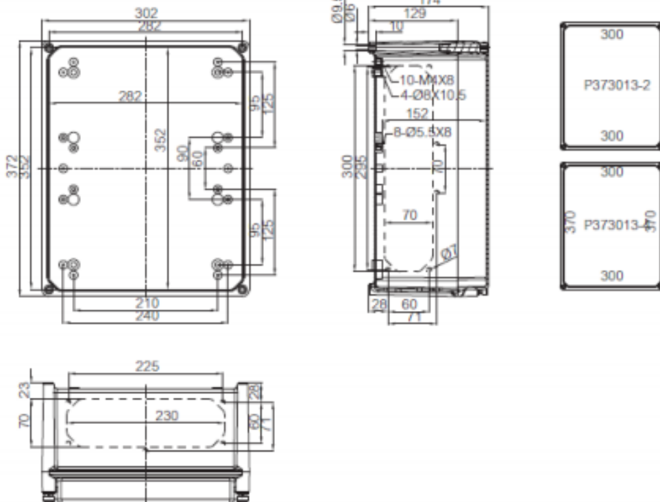
P3730 Top view - cover removed
