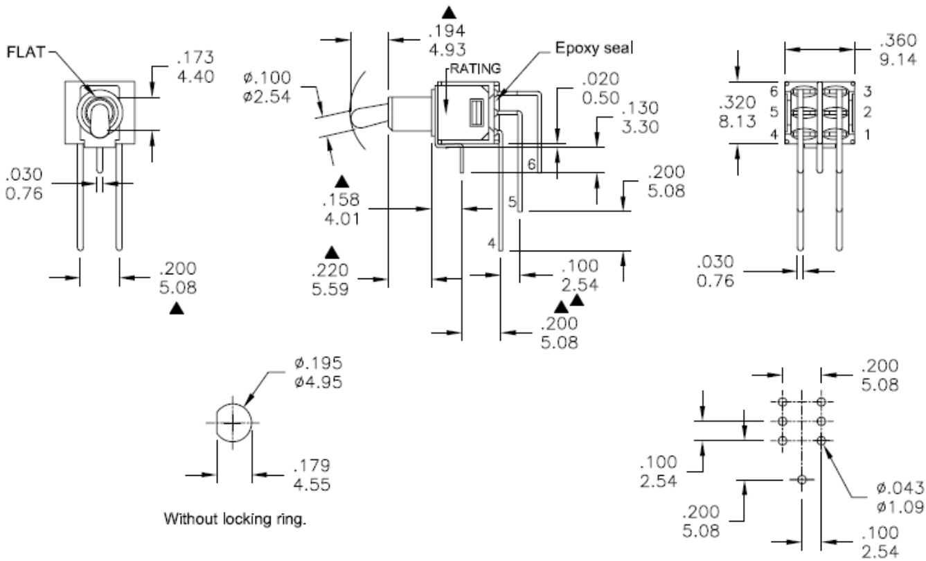
PANEL MOUNTING
