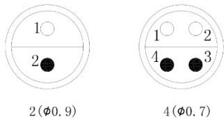
CONNECTOR SOLDER CUP VIEW
