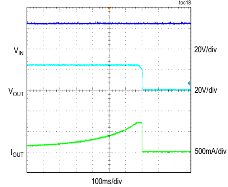
CURRENT-LIMIT RESPONSE
