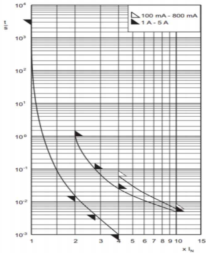
Zeit/Strom-Kennlinien Time-Current Curves
