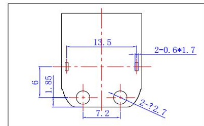
Installation hole diagram
