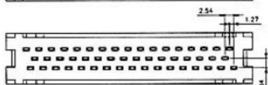
50 POSITION FEMALE
