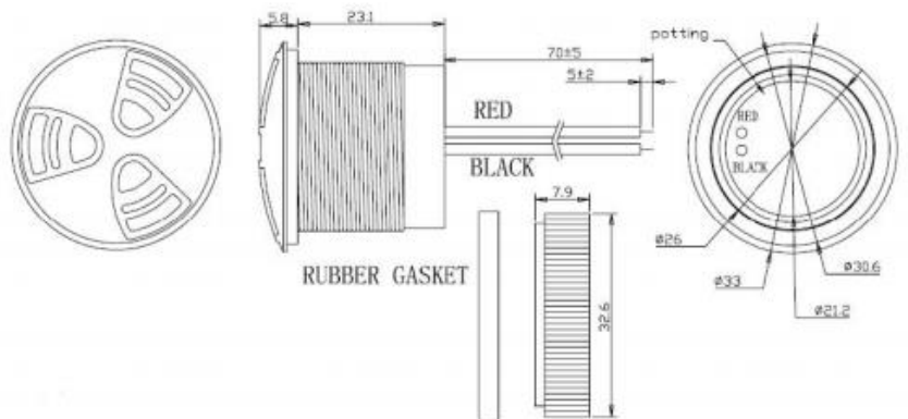
Dimensions: (mm)
