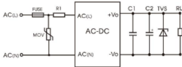
Fig. 1: Typical circuit diagram
