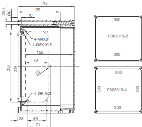
P3030 Top view - cover removed
