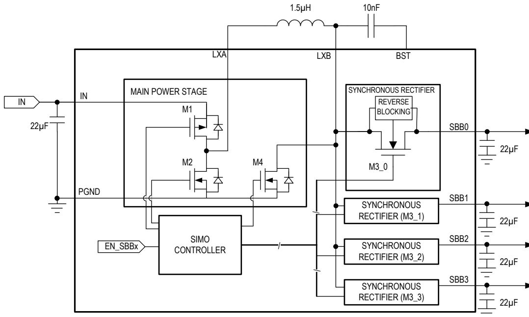
Figure 11. SIMO Simple Block Diagram
