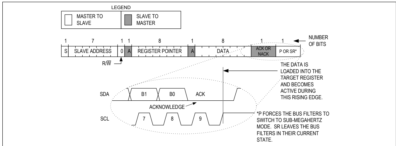
Figure 18. Writing to a Single Register with the Write Byte Protocol
