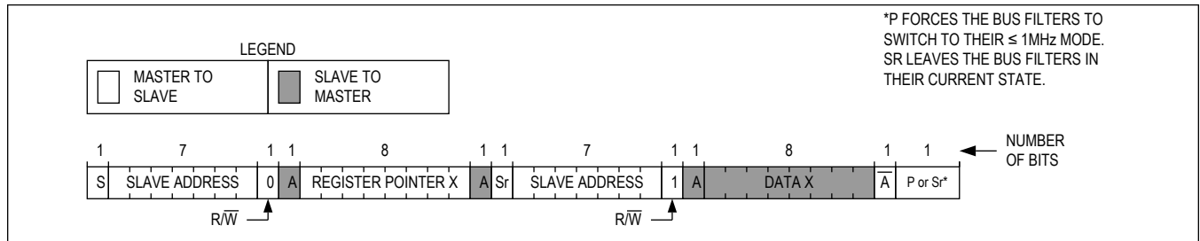
Figure 20. Reading from a Single Register with the Read Byte Protocol
