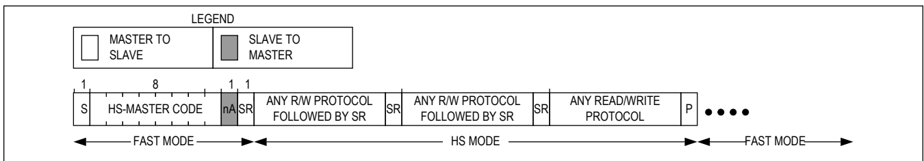
Figure 22. Engaging HS Mode
