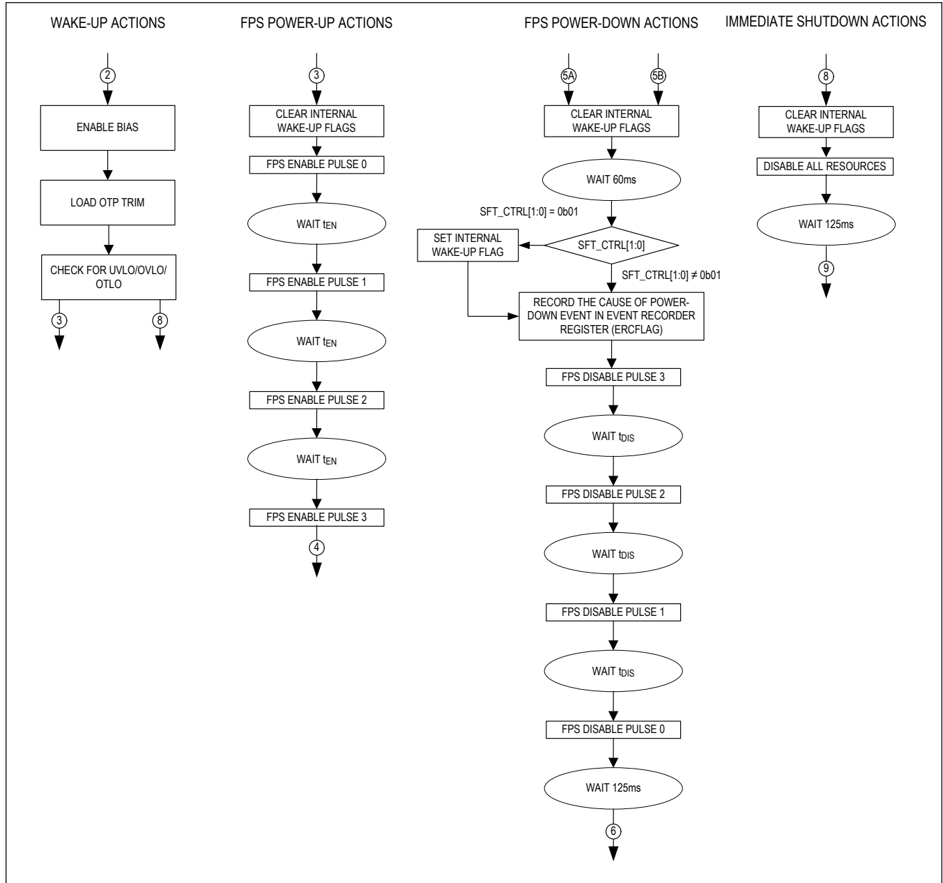
Figure 6. On/Off Controller Actions
