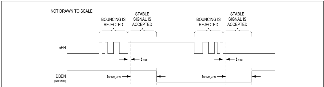
Figure 3. Debounced Input
