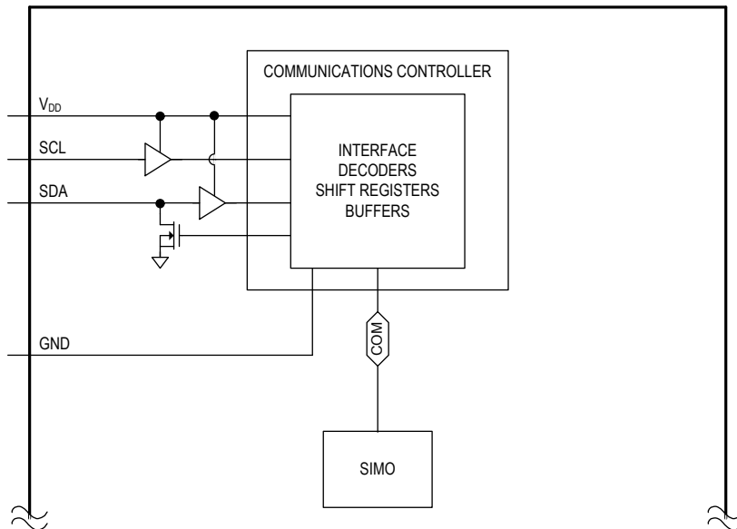
Figure 13. I 2 C Simplified Block Diagram
