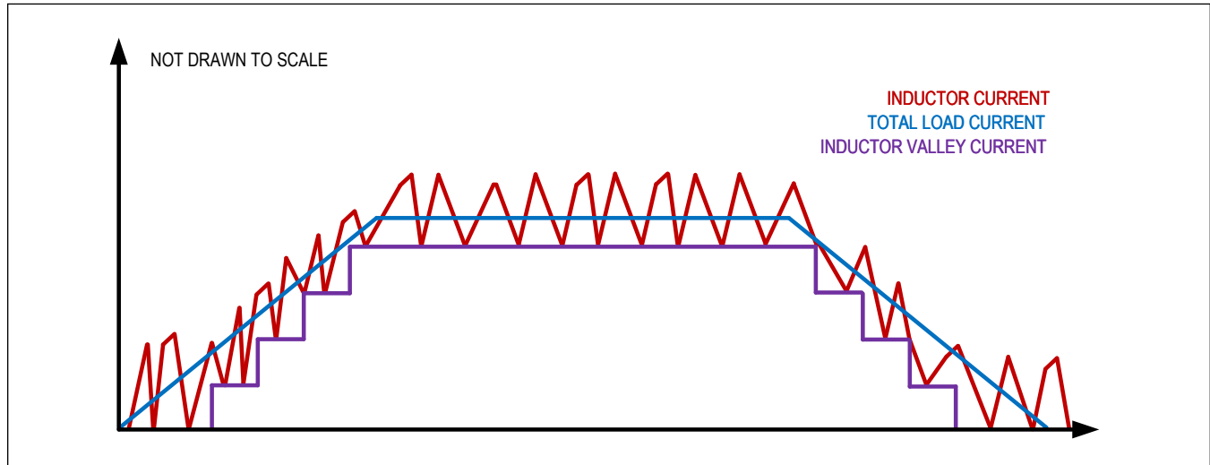
Figure 12. Valley Current Control with Changing Load Current
