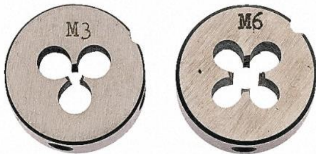
HSS Circular Dies, BS1127, Left hand thread, with split
