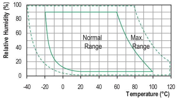
Operating conditions
