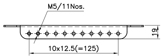
DETAIL OF MOUNTING RAIL
