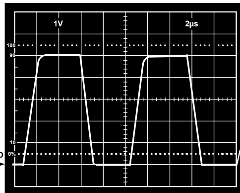
Figure 40. V_S = 5\text{ V}, 0\text{ V} ; Gain of 2 Inverter Response to 2.5 V Step, Centered -1.25\text{ V} Below Ground, R_L = 10\text{ k}\Omega
