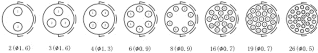
CONNECTOR SOLDER CUP VIEW
