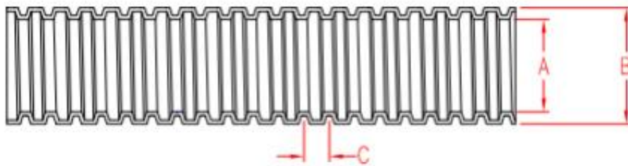
Dimensions – mm
