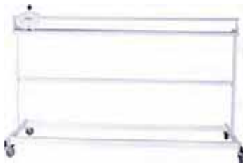
Complete mobile 120cm cutter station W154cm x D71cm x H117cm
