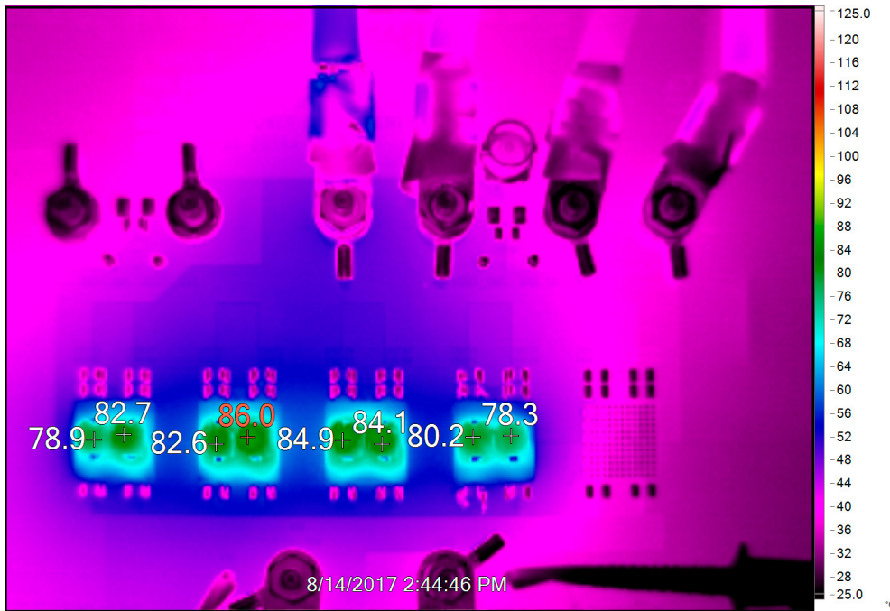
Figure 9. Thermal @ V_{IN} = 12V , V_{OUT} = 1.0V , I_{OUT} = 180A , T_A = 25^\circ C , 400LFM Airflow
