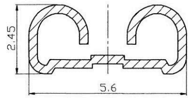
SECTION A-A SCALE 10/1
