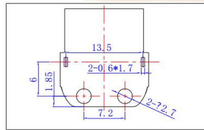
Installation hole diagram
