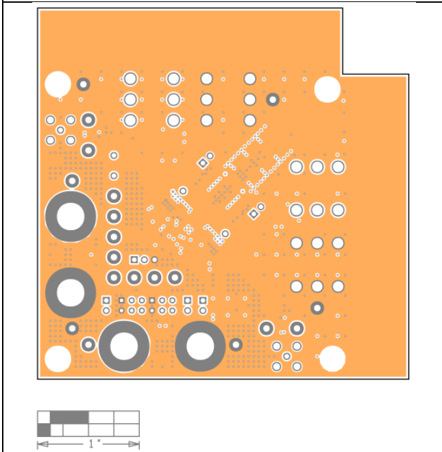
MAX20808 EV Kit PCB Layout—Layer 5
