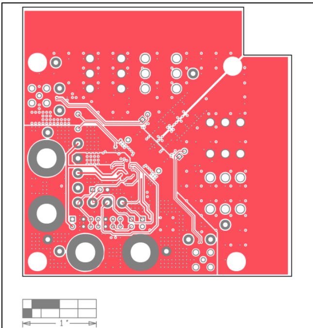
MAX20808 EV Kit PCB Layout—Layer 4
