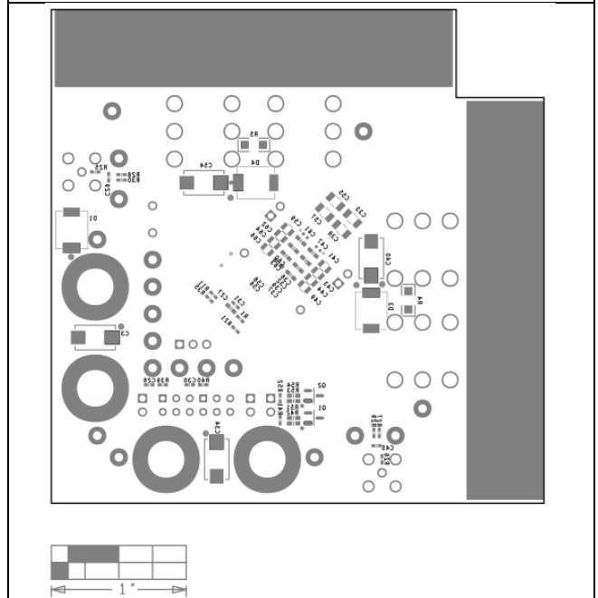
MAX20808 EV Kit Component Placement Guide—Bottom Silkscreen
