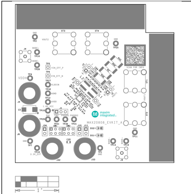
MAX20808 EV Kit Component Placement Guide—Top Silkscreen
