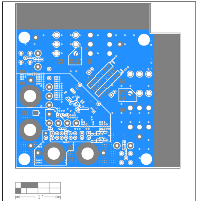
MAX20808 EV Kit PCB Layout—Bottom
