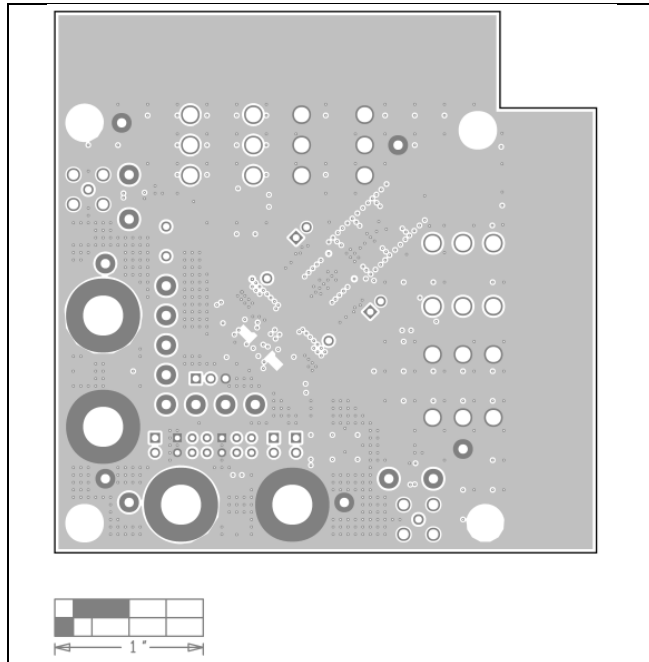
MAX20808 EV Kit PCB Layout—Layer 2
