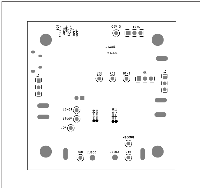
MAX77950 EV Kit Component Placement Guide—Bottom Silkscreen
