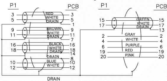
PIN Assignment
