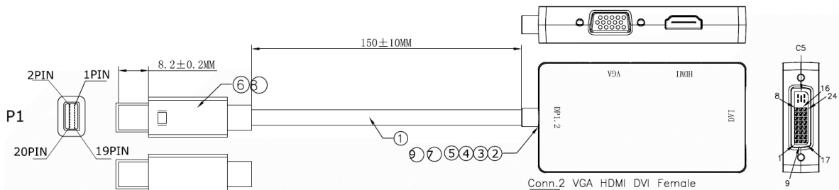
PIN Assignment
