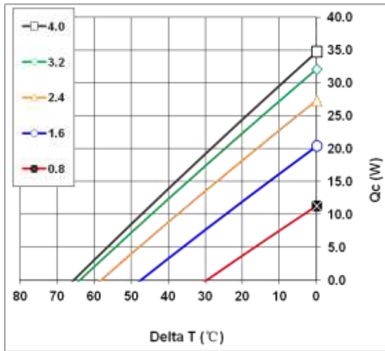
Hot Side Temperature 25°C
