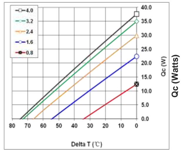
Hot Side Temperature 50°C
