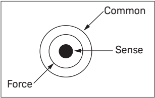
Figure 4.1. GNDU terminal
