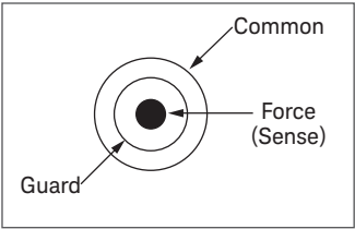
Figure 4.4. SMU terminal
