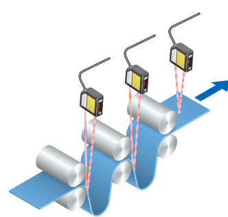
Testing sheet slack
