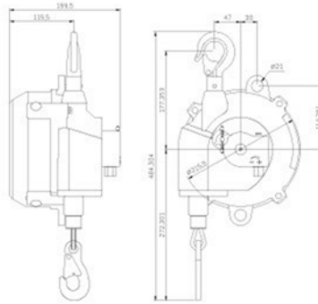
SB-60K / SB-70K
