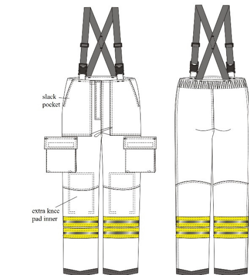
Fireman Suit 6598 EN 469:2005
