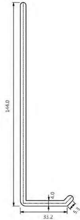
Dimensions = mm
