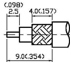
STRIPPING DIMENSION SCALE 3:1
