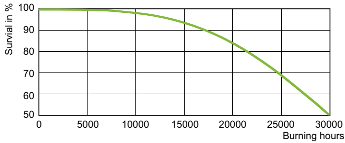
Life Expectancy Diagram - SON-T 250W E E40 1SL
