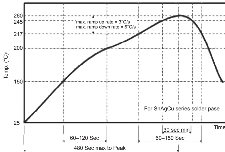
Infrared soldering profile for Chip Resistors
