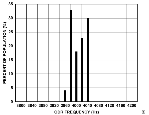
Figure 52. ADXL355 Output Data Rate (Internal Clock) Histogram
