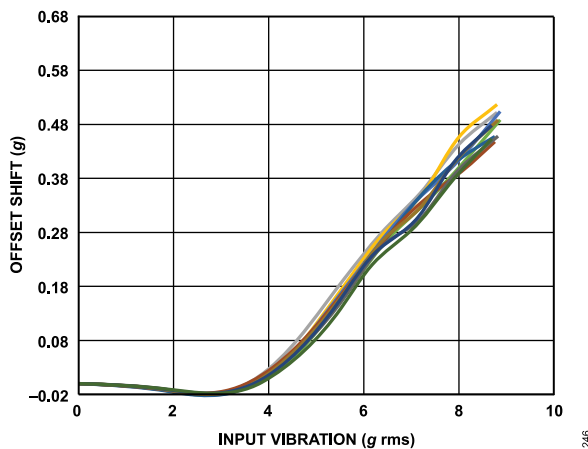
Figure 47. ADXL355 VRE, X-Axis Offset from -1 g, ±8 g Range, X-Axis Orientation = -1 g
