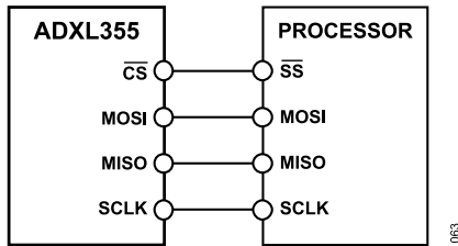
Figure 67. 4-Wire SPI Connection
