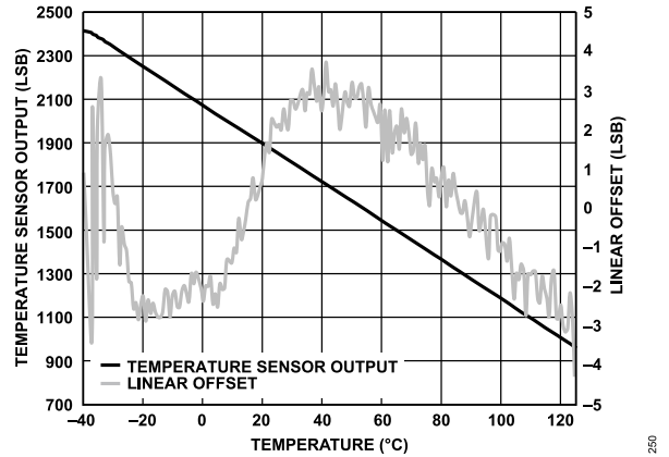
Figure 53. ADXL355 Temperature Sensor Output and Linear Offset vs. Temperature
