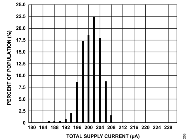
Figure 54. ADXL355 Total Supply Current, 3.3 V
