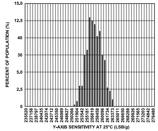
Figure 42. ADXL355 Sensitivity Histogram at 25°C, Y-Axis
