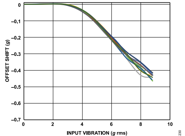
Figure 31. ADXL354 VRE, Z-Axis Offset from +1 g, ±8 g Range, Z-Axis Orientation = +1 g
