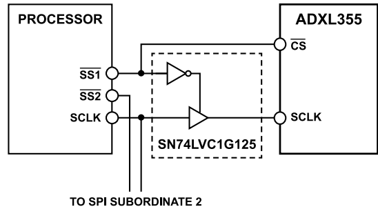
Figure 68. SCLK Protection Example
