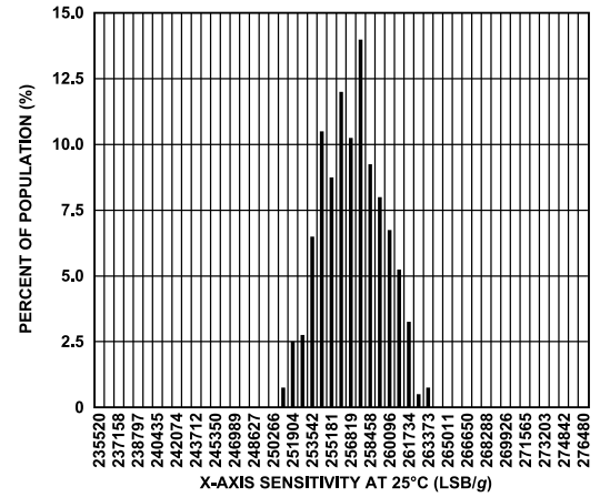
Figure 41. ADXL355 Sensitivity Histogram at 25°C, X-Axis
