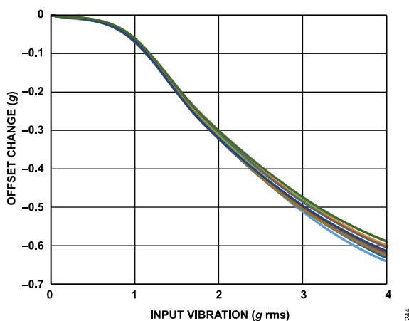
Figure 45. ADXL355 VRE, Y-Axis Offset from +1 g, ±2 g Range, Y-Axis Orientation = +1 g
