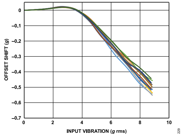
Figure 30. ADXL354 VRE, Y-Axis Offset from +1 g, ±8 g Range, Y-Axis Orientation = +1 g
