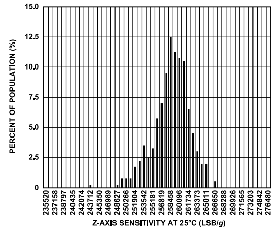
Figure 43. ADXL355 Sensitivity Histogram at 25°C, Z-Axis
