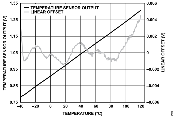
Figure 50. ADXL354 Temperature Sensor Output and Linear Offset vs. Temperature
