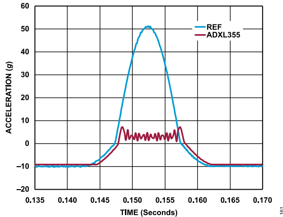
Figure 61. ADXL355 Overrange Behavior, ODR = 4 kHz
