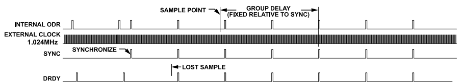
Figure 79. EXT_SYNC = 01, EXT_CLK = 1, External Synchronization, External Clock, No Interpolation Filter
