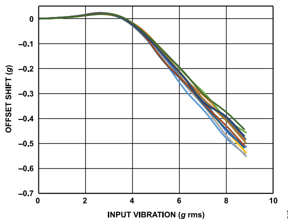
Figure 48. ADXL355 VRE, Y-Axis Offset from +1 g, ±8 g Range, Y-Axis Orientation = +1 g
