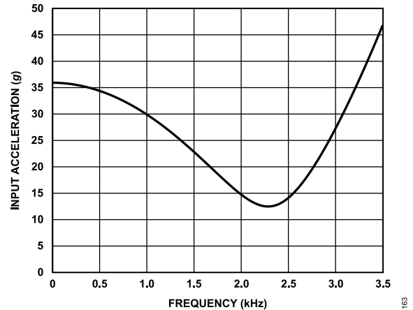
Figure 63. Z-Axis Mechanical Headroom vs. Frequency Comparison for ADXL354/ADXL355
