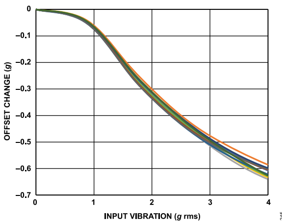
Figure 46. ADXL355 VRE, Z-Axis Offset from +1 g, ±2 g Range, Z-Axis Orientation = +1 g
