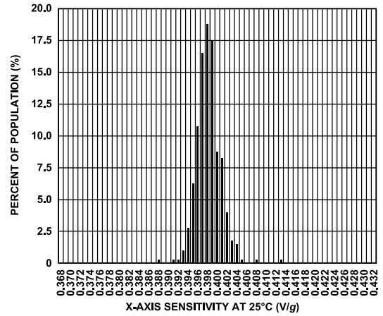
Figure 23. ADXL354 Sensitivity Histogram at 25°C, X-Axis
