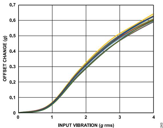
Figure 44. ADXL355 VRE, X-Axis Offset from -1 g, ±2 g Range, X-Axis Orientation = -1 g
