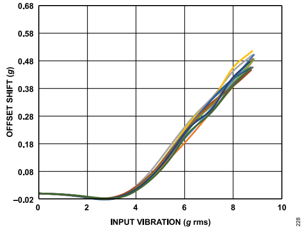
Figure 29. ADXL354 VRE, X-Axis Offset from -1 g, ±8 g Range, X-Axis Orientation = -1 g
