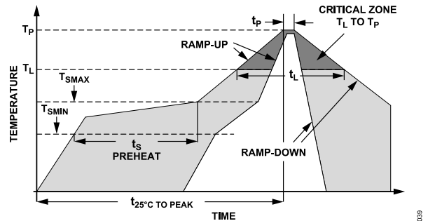
Figure 5. Recommended Soldering Profile
