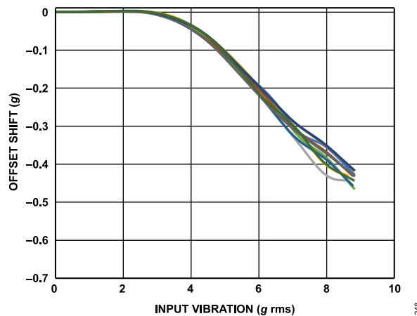
Figure 49. ADXL355 VRE, Z-Axis Offset from +1 g, ±8 g Range, Z-Axis Orientation = +1 g
