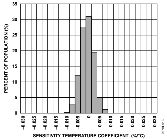
Figure 13. Y-Axis Sensitivity Temperature Coefficient, V_S = V_{DD/IO} = 3.3 V
