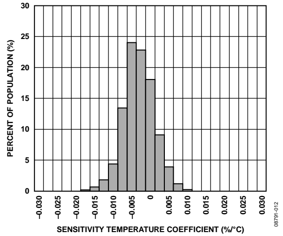
Figure 12. X-Axis Sensitivity Temperature Coefficient, V_S = V_{DD/IO} = 3.3 V
