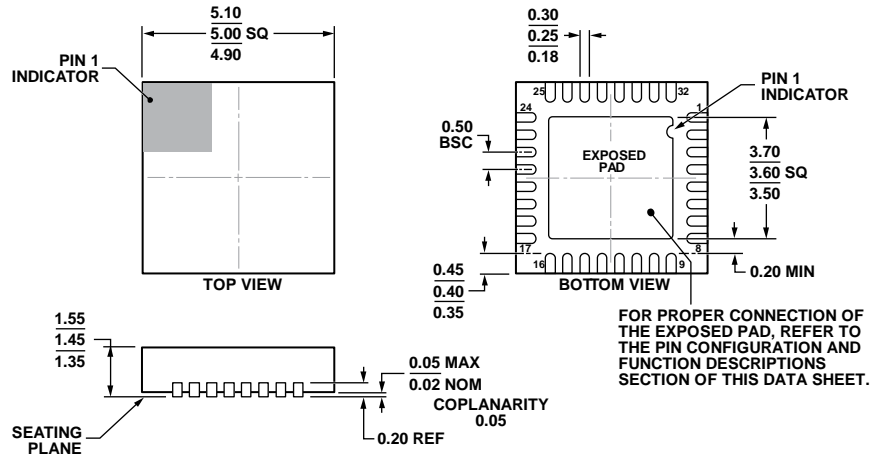
Figure 40. 32-Lead Lead Frame Chip Scale Package [LFCSP_LQ] 5 mm × 5 mm Body, Thick Quad (CP-32-17) Dimensions shown in millimeters
