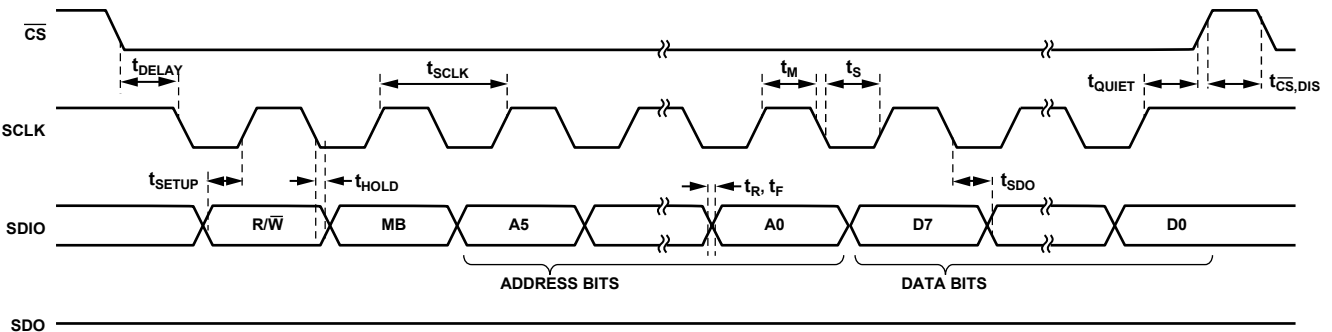
Figure 26. SPI 3-Wire Read/Write
