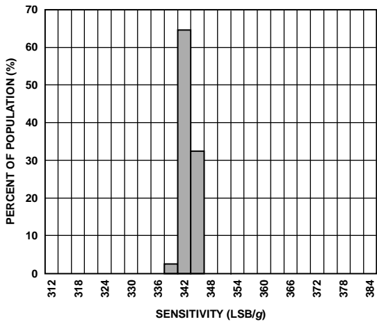
Figure 10. Y-Axis Sensitivity, V_S = V_{DD/IO} = 3.3 V , 25^\circ C
