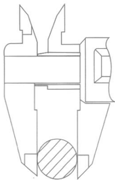
Outside Measurement
