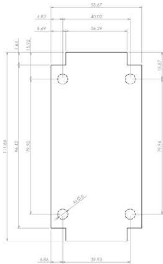
Base PCB
