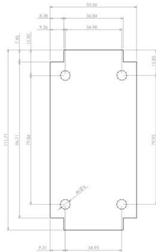
Cover PCB
