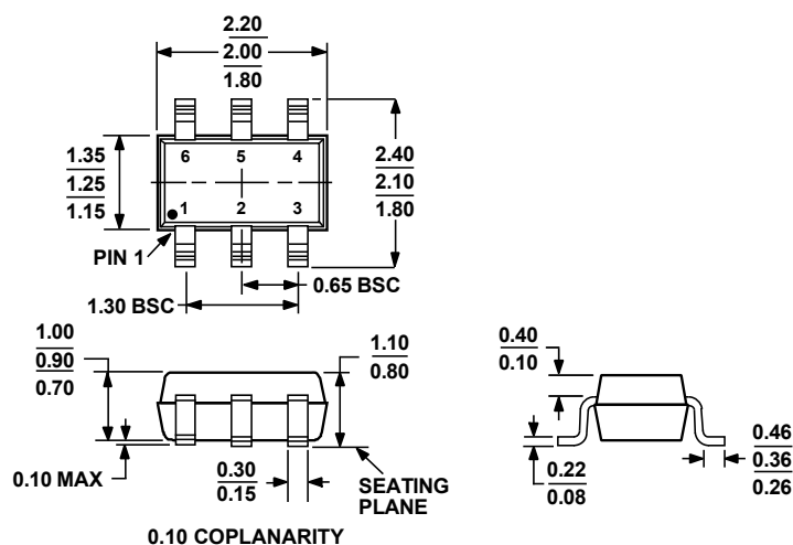
COMPLIANT TO JEDEC STANDARDS MO-203-AB Figure 59. 6-Lead Thin Shrink Small Outline Transistor Package [SC-70] (KS-6) Dimensions shown in millimeters
