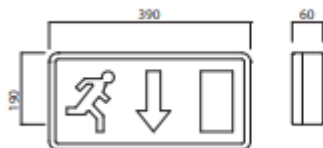
795-9748 LED Emergency exit box maintained 3Hr
