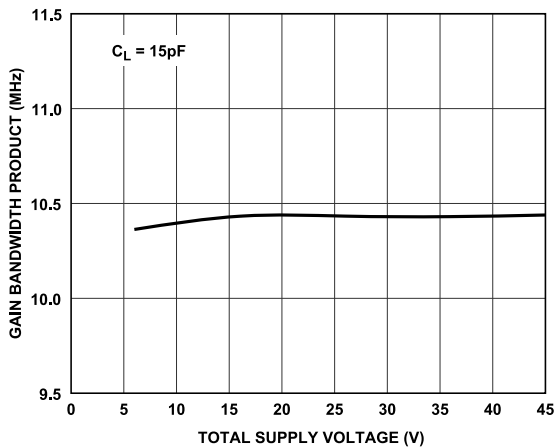
Figure 33. Gain Bandwidth Product vs. Total Supply Voltage
