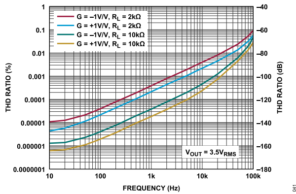
Figure 41. THD Ratio vs. Frequency
