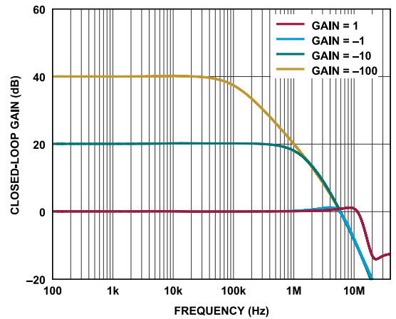
Figure 32. Closed-Loop Gain vs. Frequency
