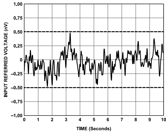
Figure 65. 0.1 Hz to 10 Hz Voltage Noise
