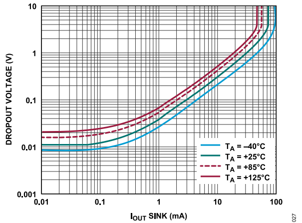
Figure 27. V_{DROPOUT}(V_{OUT} - V^-) vs. I_{OUT} Sink
