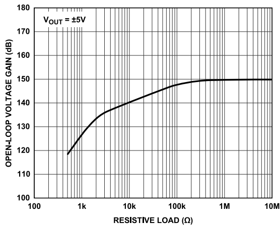
Figure 72. DC Open-Loop Gain vs. R_L
