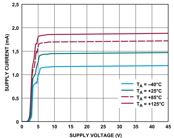
Figure 66. I_S per Amplifier vs. Supply Voltage at Various Temperatures
