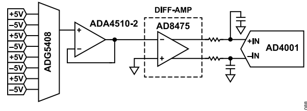
Figure 76. 16-bit, 8-Channel, Single-ended to Differential, Multiplexed Data Acquisition System
