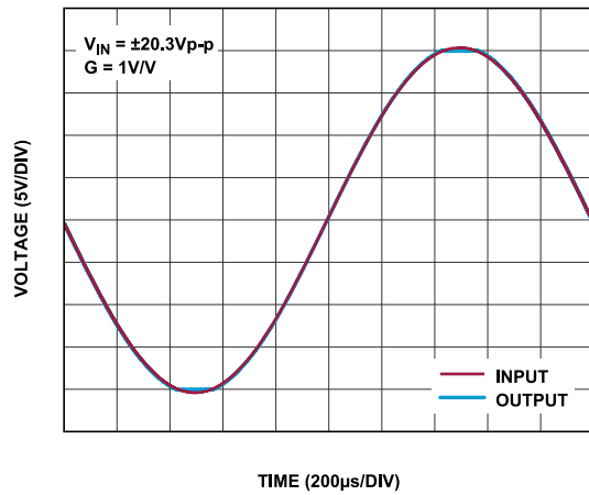
Figure 71. No Phase Reversal
