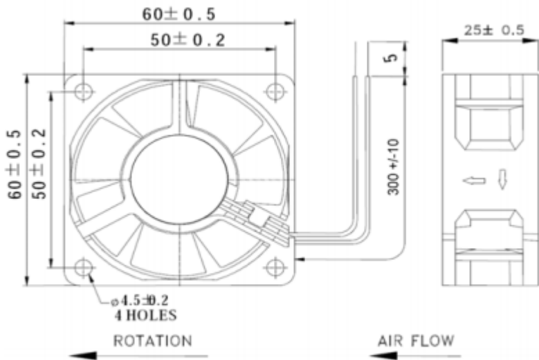
*Drawing for Dimensional Reference Only
