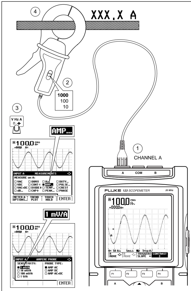
Figure 3. ScopeMeter Setups
