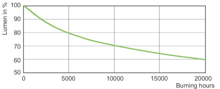
Lumen Maintenance Diagram - HPI PLUS 400W/645 BU E40 1SL/6
