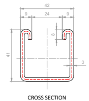
CROSS SECTION
