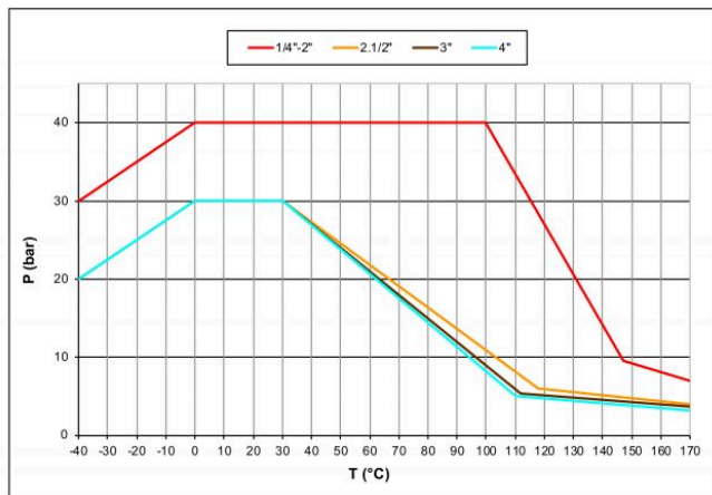
Pressure-temperature chart
