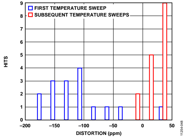
Figure 45. Thermal Hysteresis
